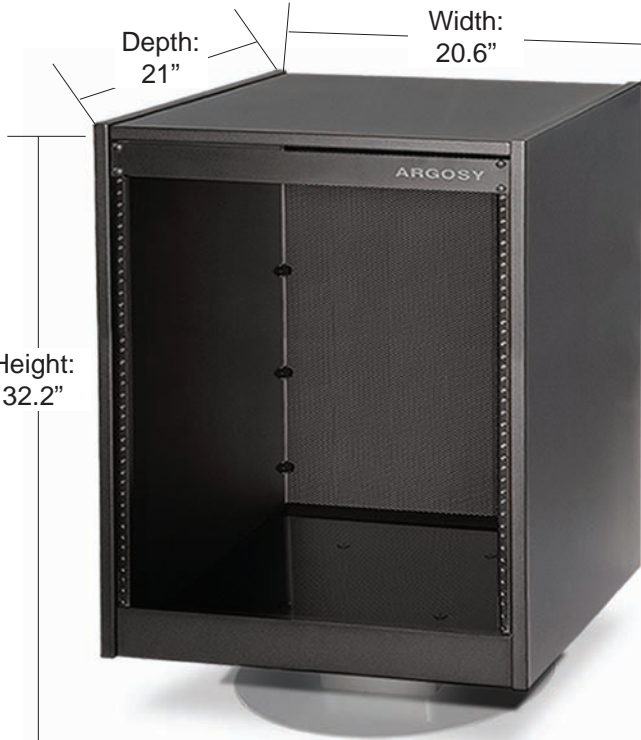
Mirage R14 14 RU Spaces Internal Depth: 20"
