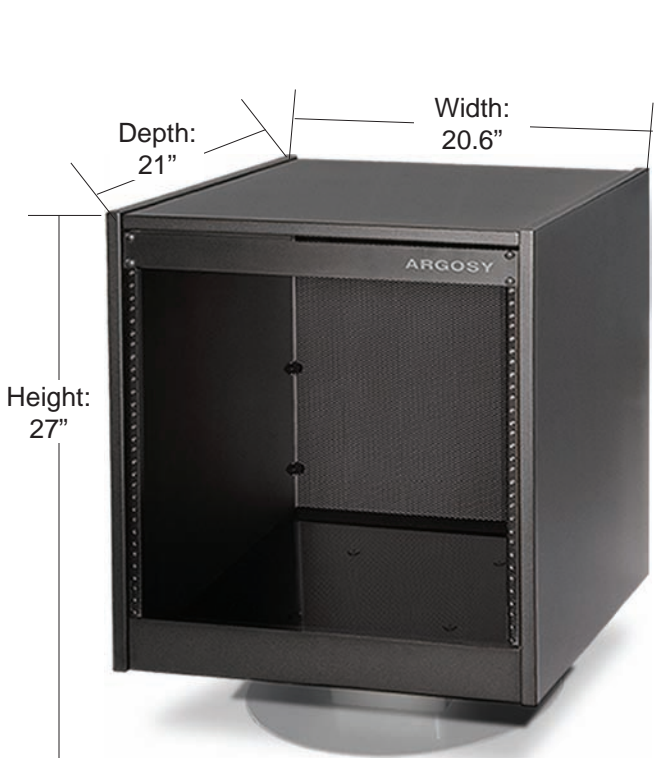
Mirage R11 11 RU Spaces Internal Depth: 20"
