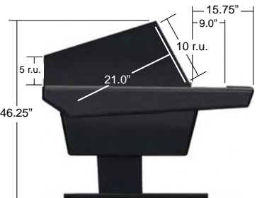
V Series profile with V1005 rack module.
