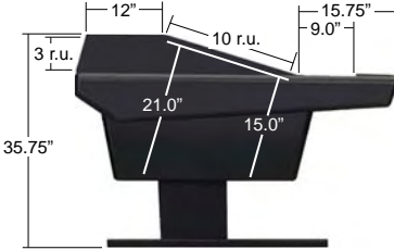
V Series profile with V1003 rack module.
